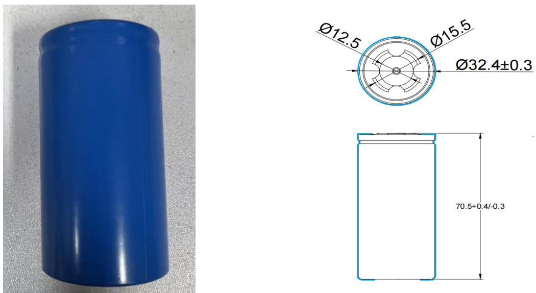
电池包膜后图片和外形尺寸 Cell's appearance and dimension with PVC sleeve
