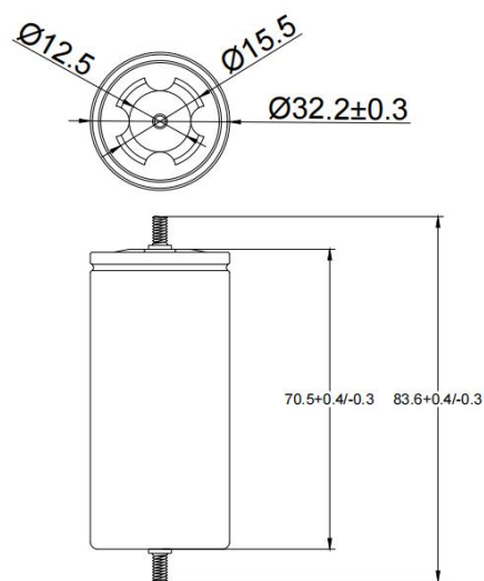
丝柱电池图片和外形尺寸 The Cell's with welded screw appearance and dimension
