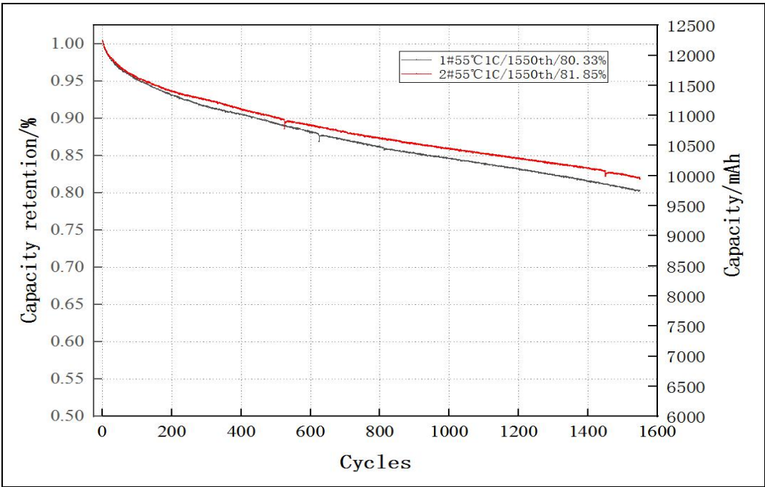
6.0 Ah 磷酸铁锂电池 55±2℃ 1C 循环曲线图 (A+) 55±2℃ 1C cycle curve of 6.0 Ah LiFePO 4 cell (A+)
