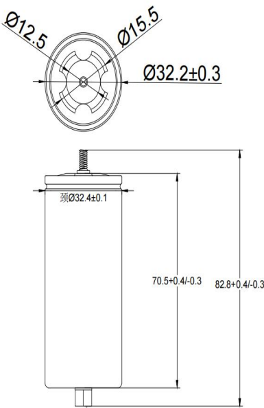
丝柱电池图片和外形尺寸 The Cell's with welded screw appearance and dimension
