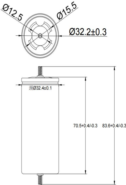
丝柱电池包膜后图片和外形尺寸 The Cell's with welded screw appearance and dimension with PVC sleeve
