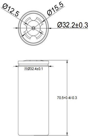
电池图片和外形尺寸 Cell's appearance and dimension
